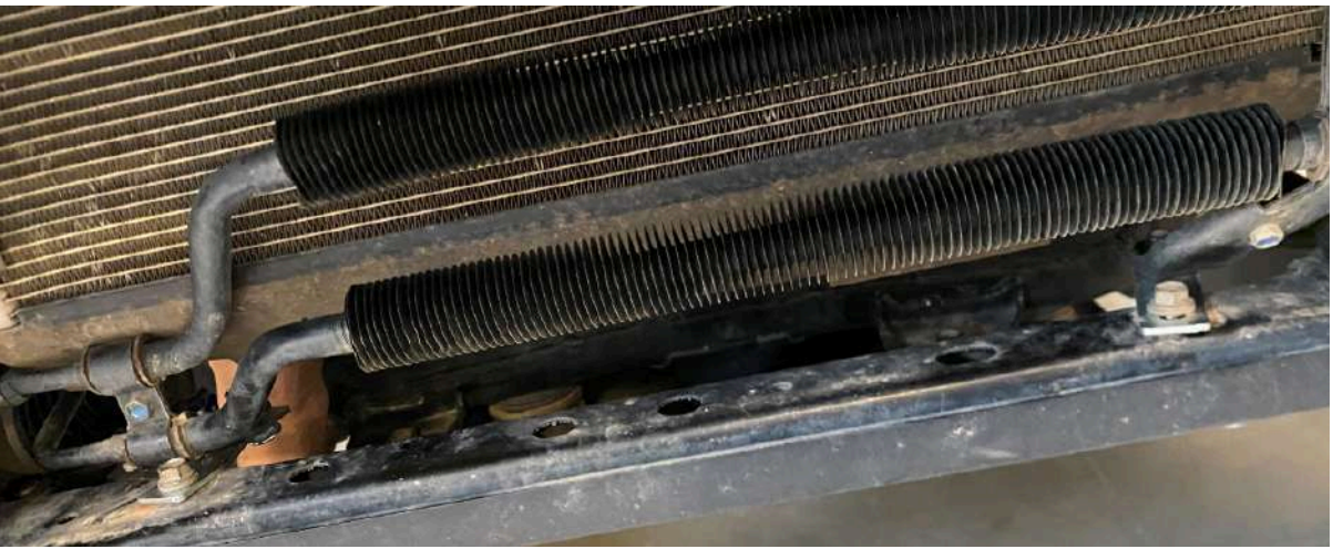
Figure 17: Correct installation of frontmost brackets.
