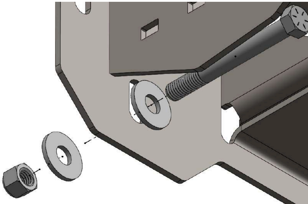
Figure 23: Hardware orientation
